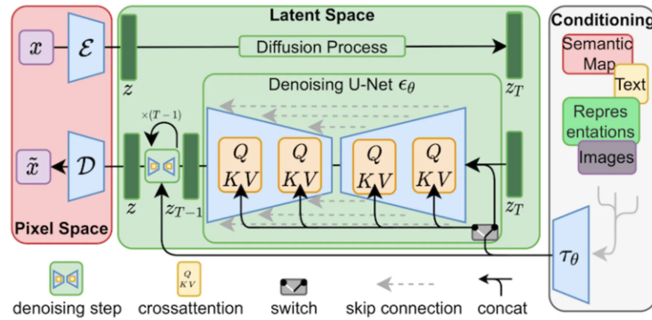
FIGURE 2 – Latent Diffusion Model
